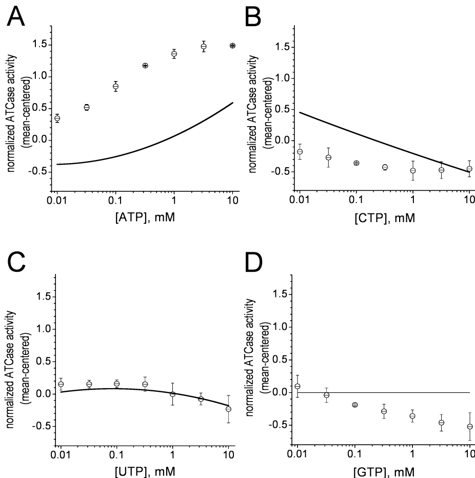
FIGURE 1: Comparison of effects of isolated single NTPs on ATCase activity (○; error bars are \pm 1 standard deviation of the mean of N = 2 measurements) to first-order HDMR functions of the NTPs (—): (A) f_1 ([ATP]), (B) f_2 ([CTP]), (C) f_3 ([UTP]), and (D) f_4 ([GTP]). The y axis shows normalized ATCase activity; one normalized activity unit refers to the activity of ATCase in the absence of any NTP. Consistent with the RS–HDMR framework (in which all component functions are added to the mean measured ATCase activity to obtain the estimated activity), the y axis values are mean-centered: the mean ATCase activity obtained in the experiments involving random concentration combinations of all four nucleotides ( f_0 = 0.78 ) has been subtracted from the observed experimental values for the isolated single nucleotides. The use of a thin line to depict f_4 (GTP) reflects the lack of a significant first-order effect of GTP.
