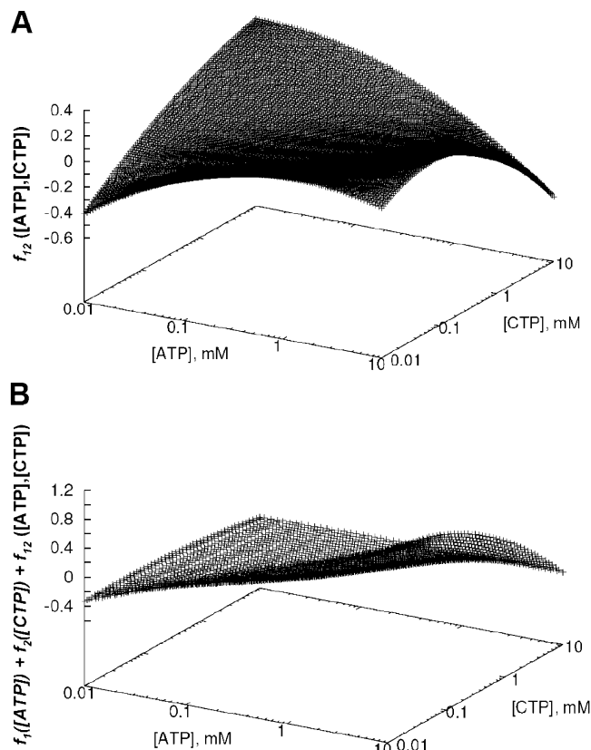
FIGURE 2: Second-order effect of ATP \times CTP. (A) Second-order RS-HDMR component function f_{12}([ATP],[CTP]) , which reflects the pairwise cooperative effect of the two nucleotides. (B) Best overall estimate of the combined effects of ATP and CTP: f_1([ATP]) + f_2([CTP]) + f_{12}([ATP],[CTP]) . z axis units in both panels are normalized ATCase activity (as per the y axis of Figure 1).
